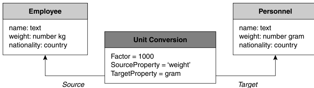
Fig. 1. Simple example of ontology mapping.
