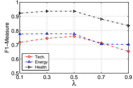
Figure 10: Performance of TFGM by varying parameter \lambda .
